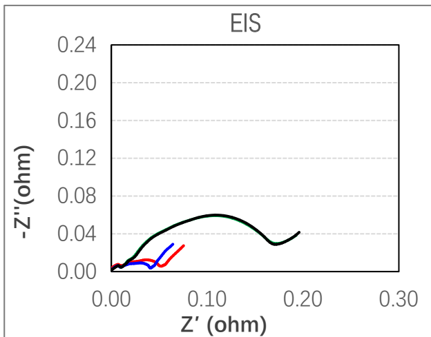
Electrochemical Impedance
