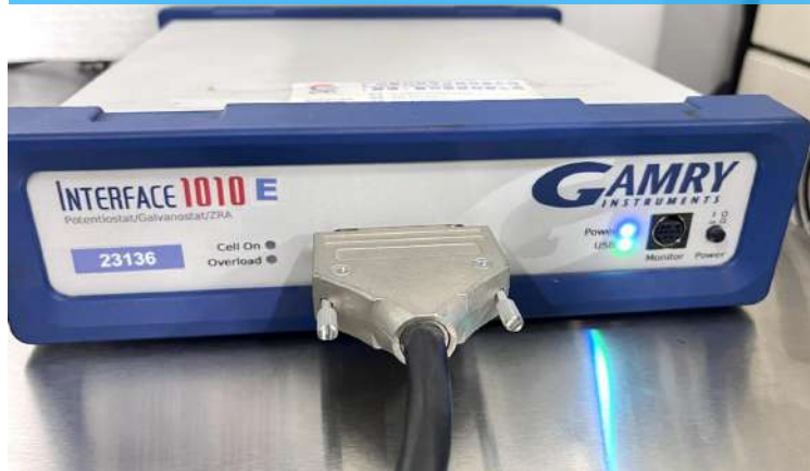
Electrochemical workstation
