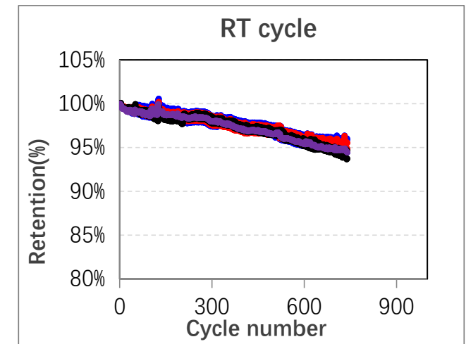
Cycling Test
